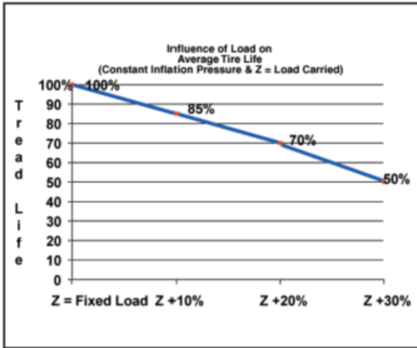
Fig. 1-56: Influence of Load on Average Tread Life
